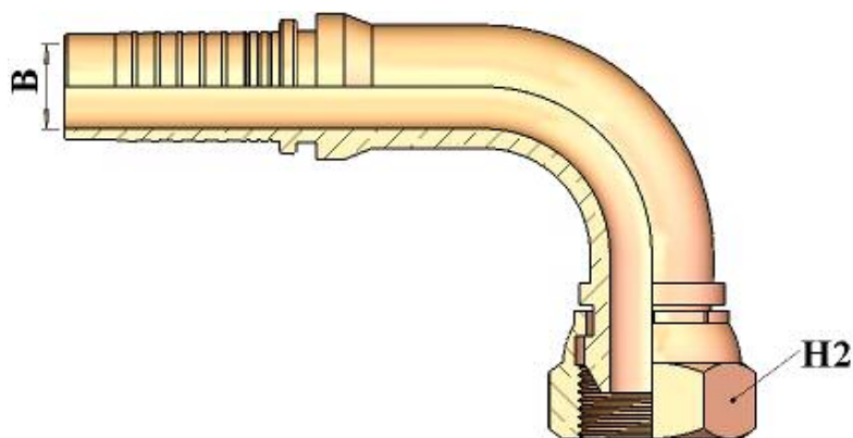
HT20591 90° BSP SWEPT ELBOW 60° CONE
