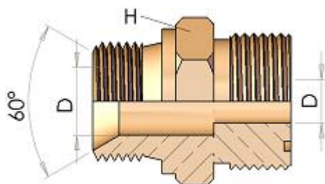
HT500524 STRAIGHT ADAPTOR BSP MALE O'RING / ORFS MALE
