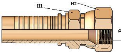
HT24011 JAPANESE METRIC FEMALE JIS (TYPE K)
