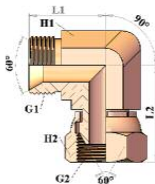
HT580405 90° ELBOW ADAPTOR BSP MALE / BSP FEMALE (C/B NUT)
