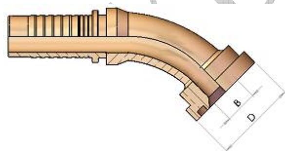
HT24145 45° JIS FLANGE (JAPANESE TYPE)
