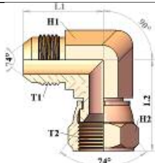
HT582525 90 ELBOW ADAPTOR JIC MALE 74° CONE /FEMAL JIC
