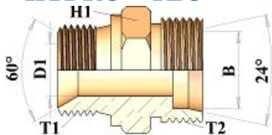
HT500515 STRAIGHT ADAPTOR BSP MALE O'RING / METRIC MALE
