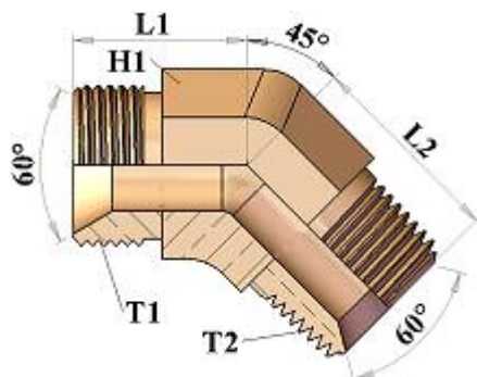
HT530407 45° ELBOW ADAPTOR BSP MALE / BSPT MALE
