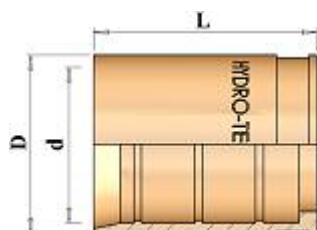
HT00820 SWAGED FERRULE FOR HOSE SIMILAR TO SAE 100 R7 AND R8
