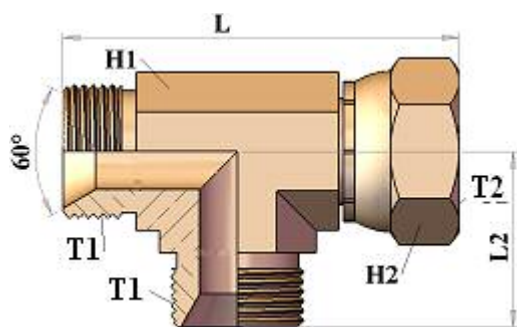
HT720405 RUN TEE BSP MALE / BSP FEMALE
