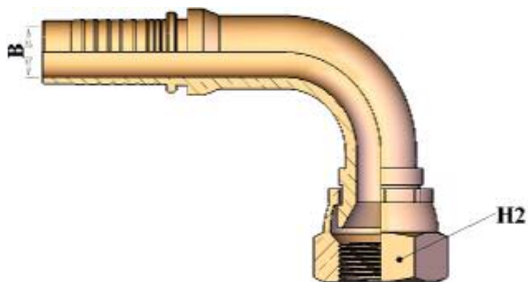
HT24091 90° JAPANESE METRIC JIS (TYPE K)
