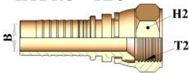
HT22511 JIC FEMALE 74° CONE SEAT
