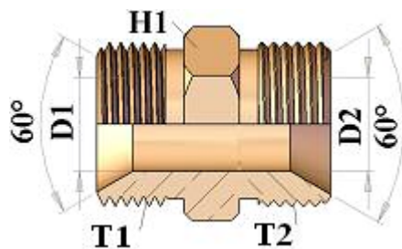
HT500404 STRAIGHT ADAPTOR MALE / BSP MALE
