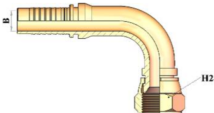
HT22591 90° JIC SWEPT ELBOW 74° CONE
