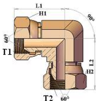
HT570505 90° ELBOW ADAPTOR BSP FEMALE / BSP FEMALE (C/B NUT)
