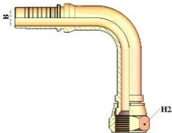
HT24791 90° JIC LONG SWEPT ELBOW 74° CONE
