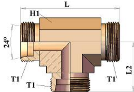
HT701515 UNION TEE ADAPTOR METRIC MALE
