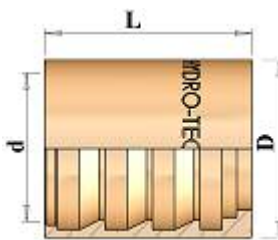
HT00110 SWAGED FERRULE FOR SAE 100 R1A DIN 2022 1ST HOSE SKIVE
