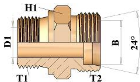
HT500615 STRAIGHT ADAPTOR BSP MALE FLAT / METRIC MALE
