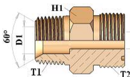
HT500724 STRAIGHT ADAPTOR BSPT MALE / ORFS MALE
