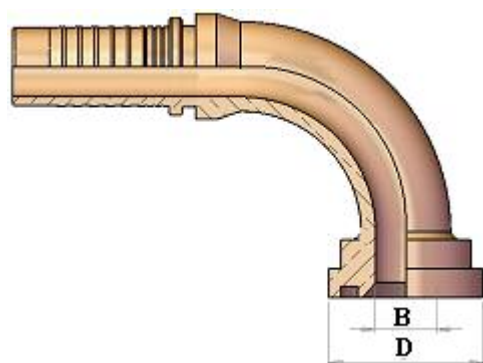
HT24190 90° JIS FLANGE (JAPANESE TYPE)
