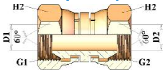
HT510505 STRAIGHT ADAPTOR BSP FEMALE / BSP FEMALE (C/B NUT)
