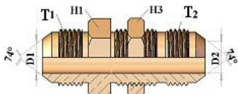
HT502523 STRAIGHT BULKHEAD ADAPTOR JIC MALE 74° CONE
