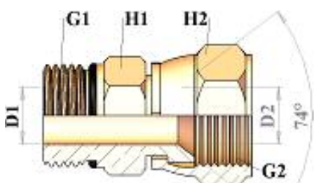
HT523025 STRAIGHT ADAPTOR SEA O'RING MALE / JIC FEMALE
