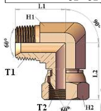
HT580705 90° ELBOW ADAPTOR BSPT MALE / BSP FEMALE (C/B NUT)
