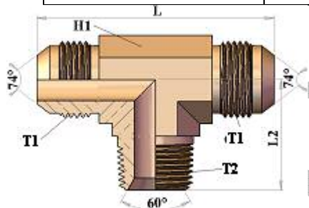
HT702507 BRANCH TEE ADAPTOR JIC MALE / BSPT MALE 74° CONE
