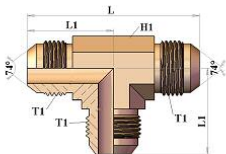
HT702525 UNION TEE ADAPTOR JIC MALE 74° CONE
