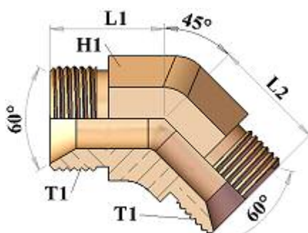
HT530404 45° ELBOW ADAPTOR BSP MALE / BSP MALE
