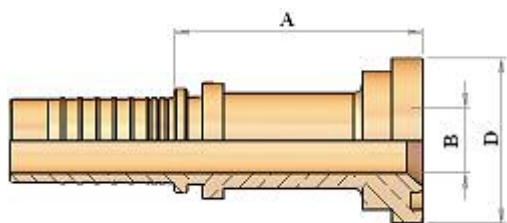
HT24111 STRAIGHT JIS FLANGE (JAPANESE TYPE)
