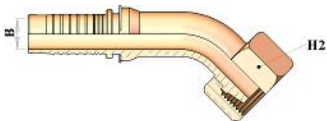
HT21343 45° METRIC SWEPT ELBOW MULTISEAL FEMALE DIN 3868
