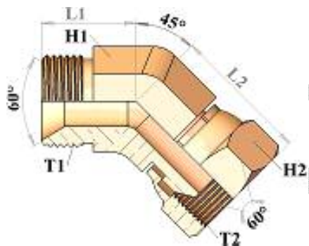
HT550405 45° ELBOW ADAPTOR BSP MALE / BSP FEMALE
