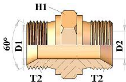
HT500505 STRAIGHT ADAPTOR BSP MALE / BSP MALE
